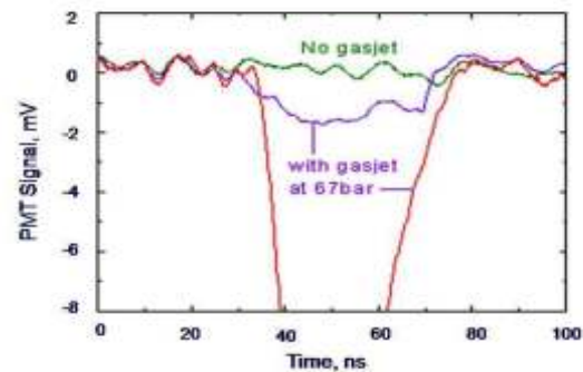
Fig.L.1.2 : Scintillator-PMT signals showing presence of electrons accelerated to energy exceeding 70 MeV.
