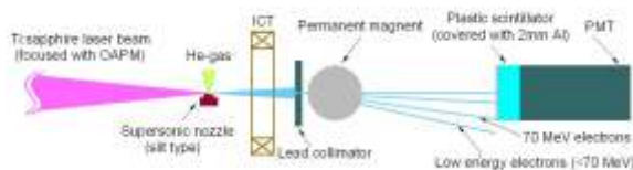
Fig.L.1.1 : Set-up of the electron acceleration experiment
